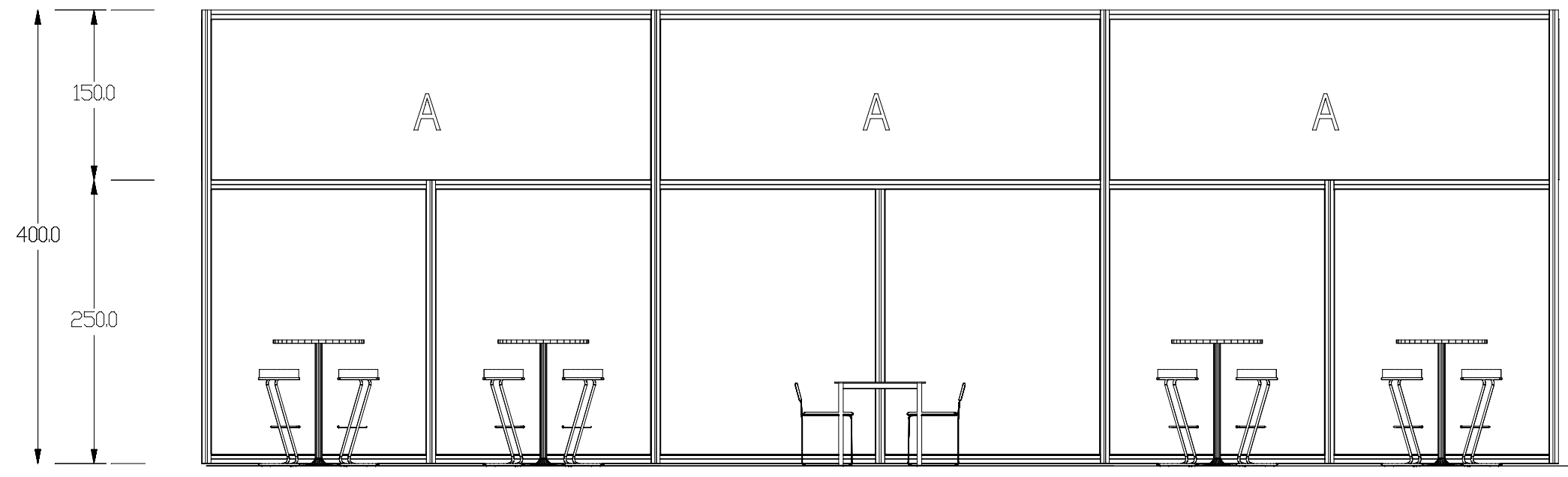
FRONT VIEW
