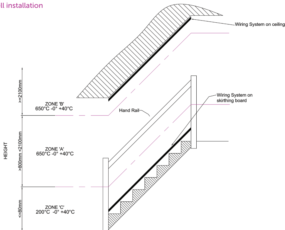
Figure 4: Stairwell installation
