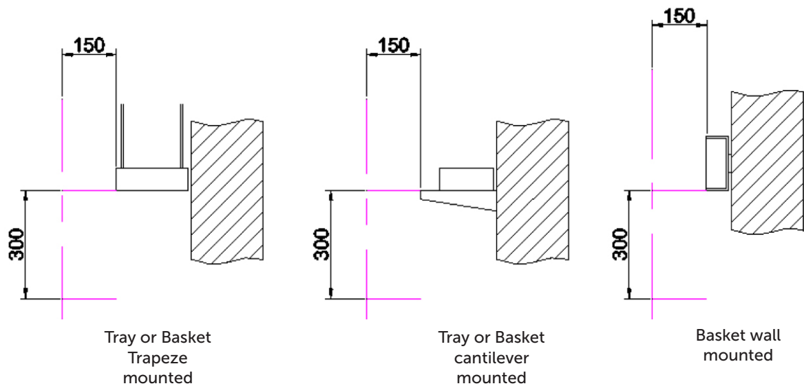
Figure 6: Tray, Ladder and Basket Examples
