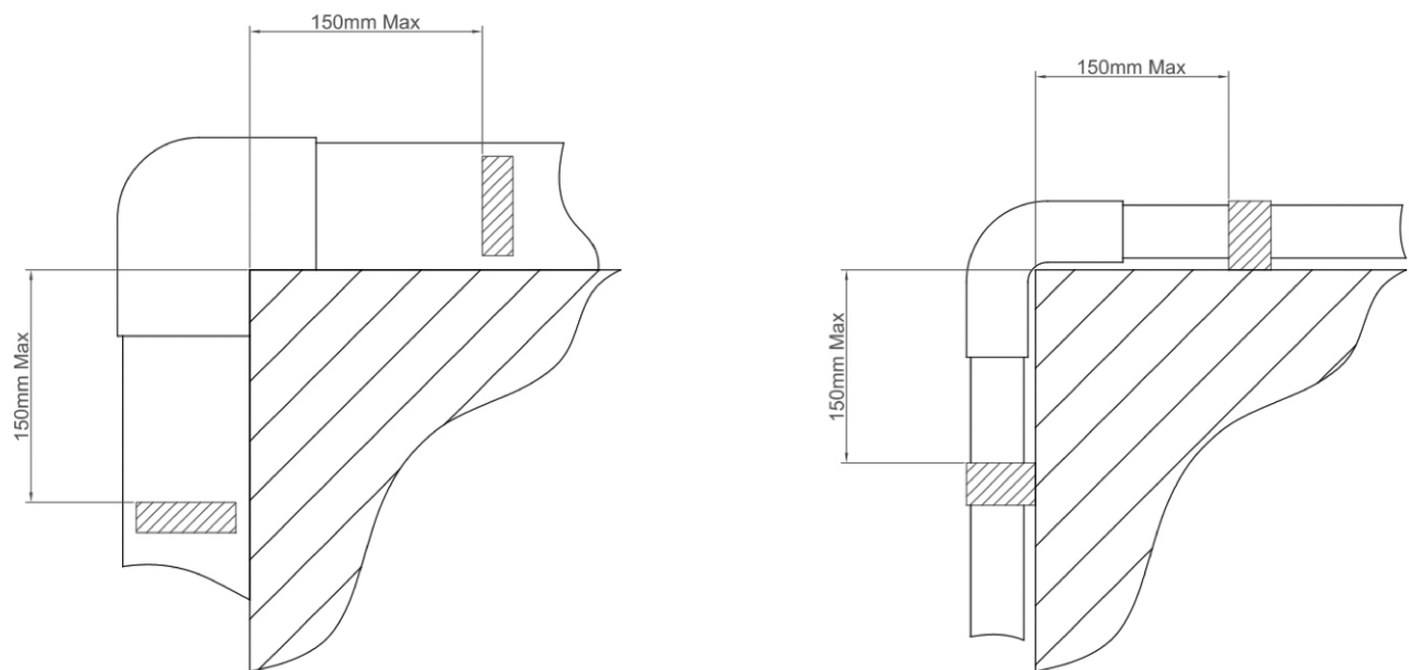
Figure 9: Trunking and Conduit – External Bends
