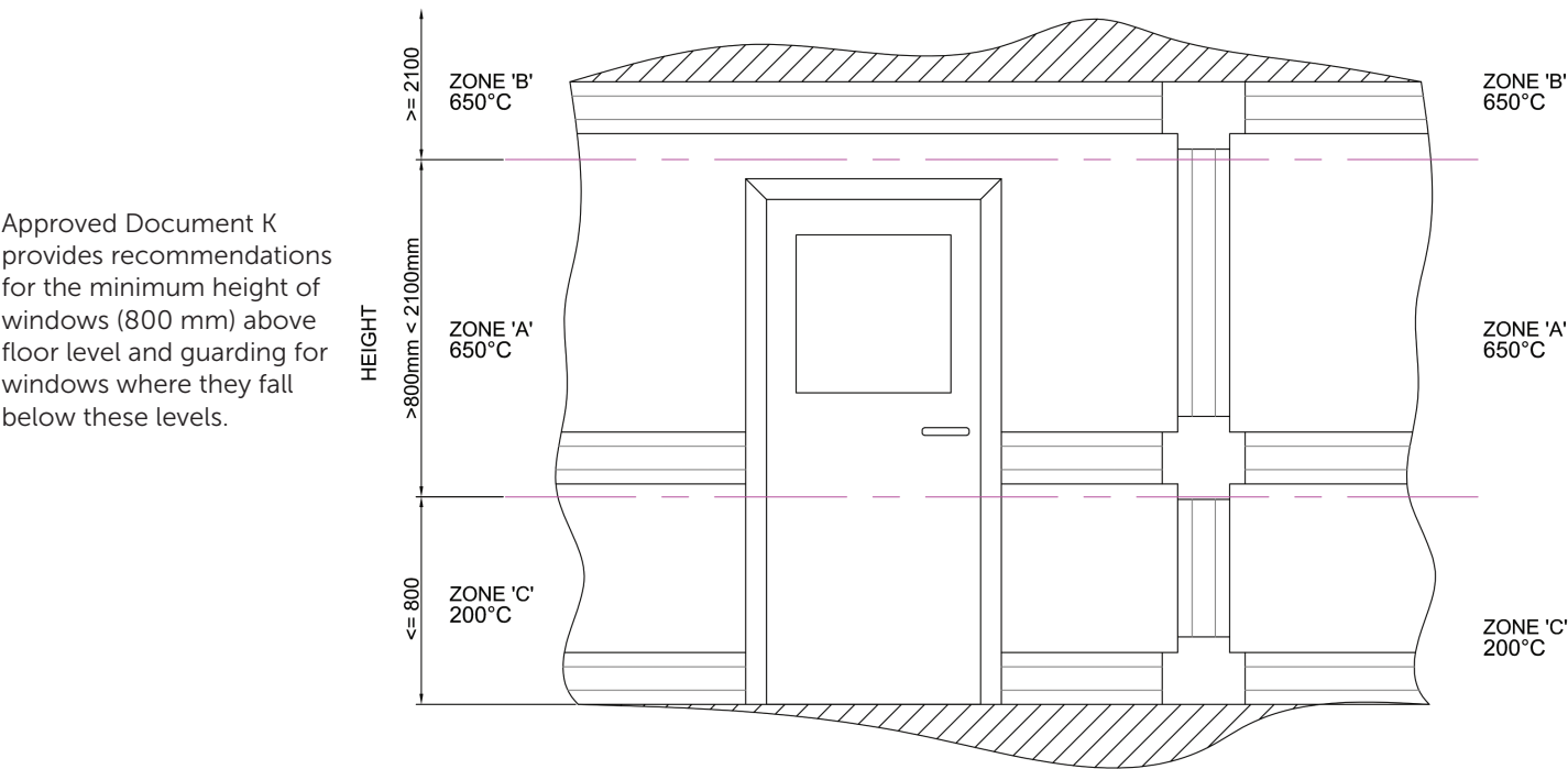
Figure 1 – Installation Zones A, B & C
