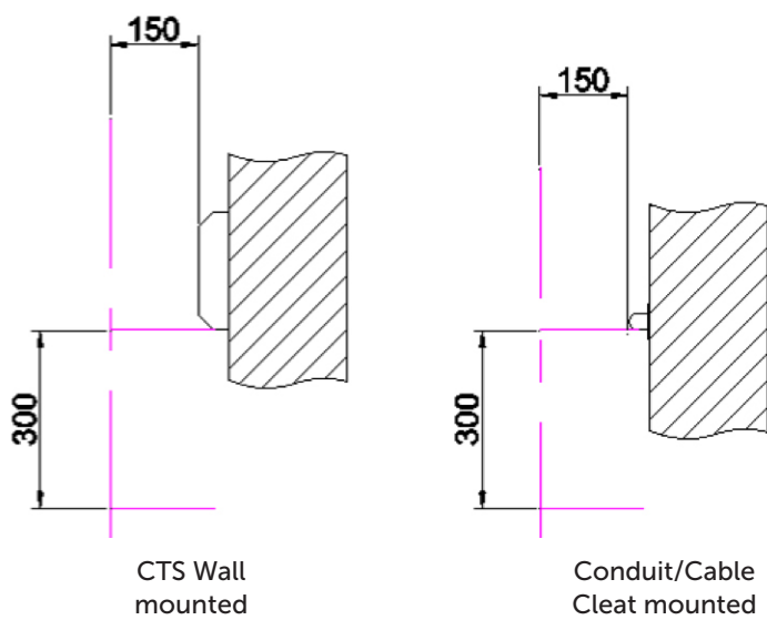
Figure 7: Trunking and Conduit – Horizontal runs on vertical face
