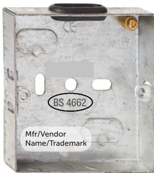
Figure 1. Example of a flush back box marked with BS 4662
