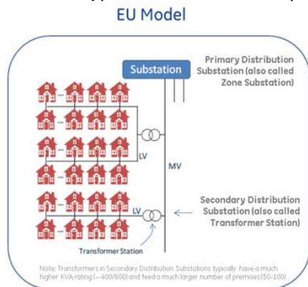
Picture 1 Typical structure of European most common model of MV network
