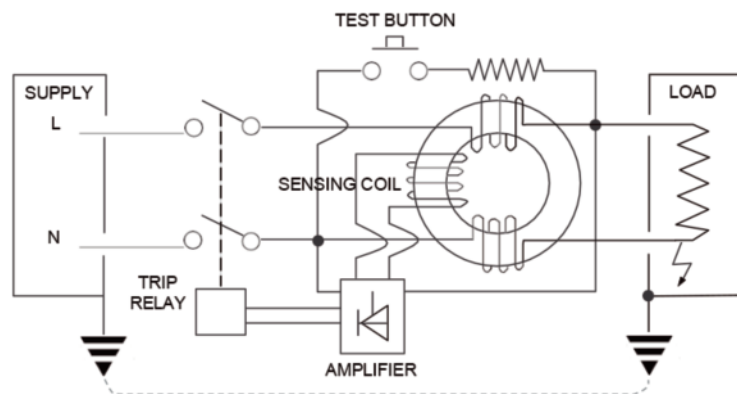
FIGURE 23 – VOLTAGE DEPENDENT RCD DESIGN
