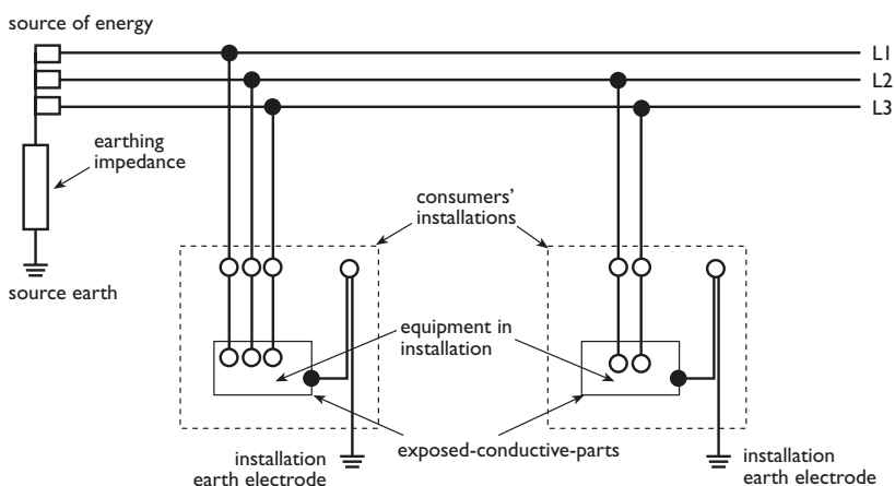
FIGURE 12 –IT SYSTEM
