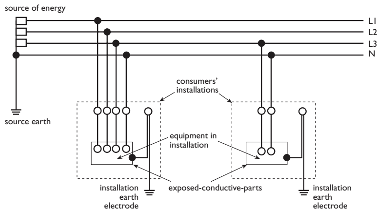
FIGURE 11 –TT SYSTEM
