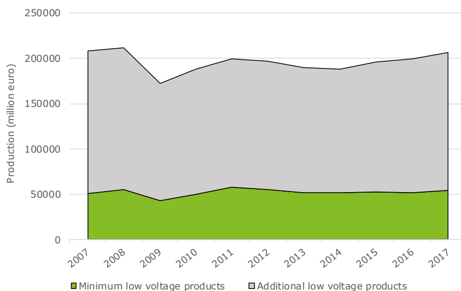
Figure 5 – EU28 production of low voltage products, 2007-2017
