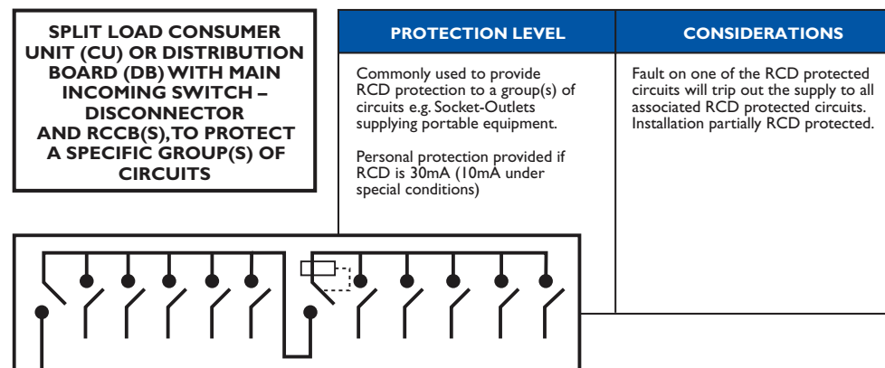
Figure 16 Split load protection (A)
