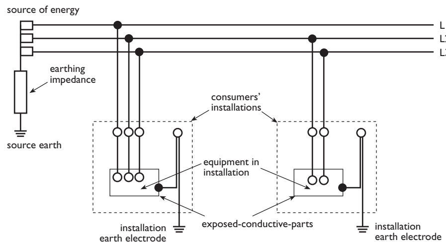
Figure 12 IT System
