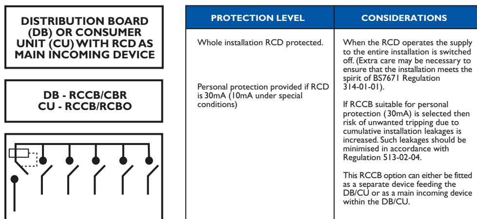
Figure 15 Whole installation protection
