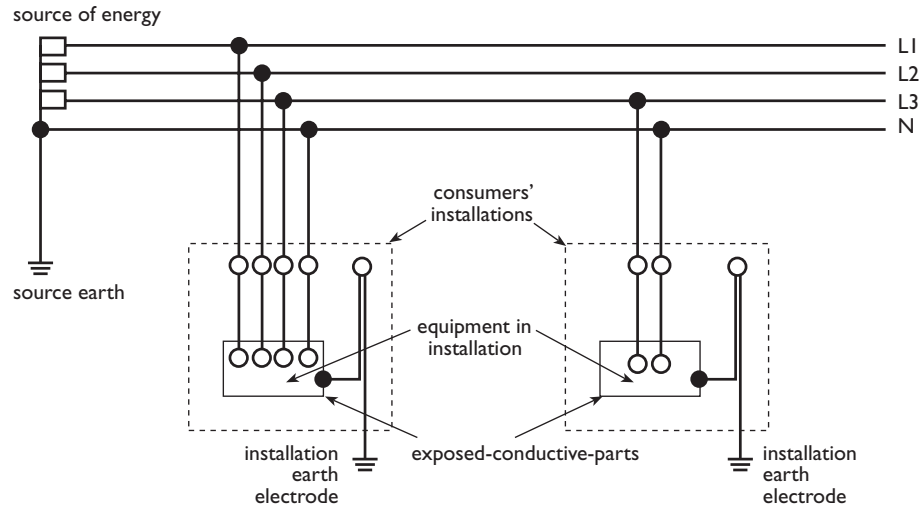
Figure 11 TT System
