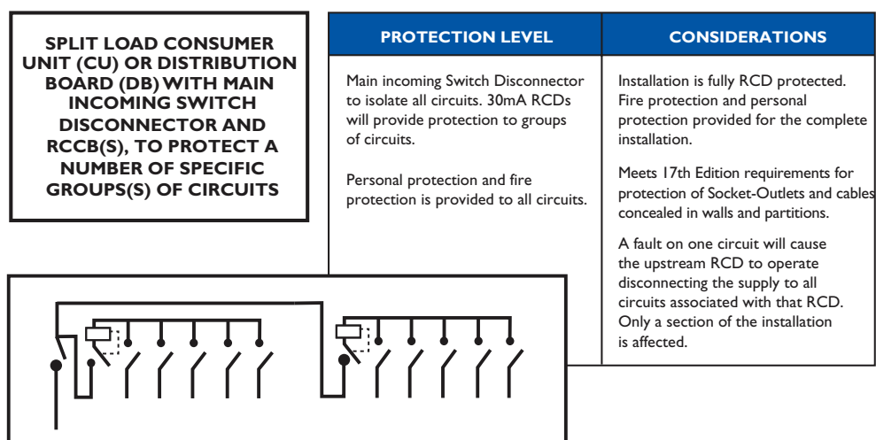
Figure 17A Dual Split load protection (C)
