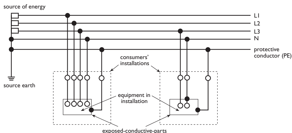
Figure 9 TN-S System
