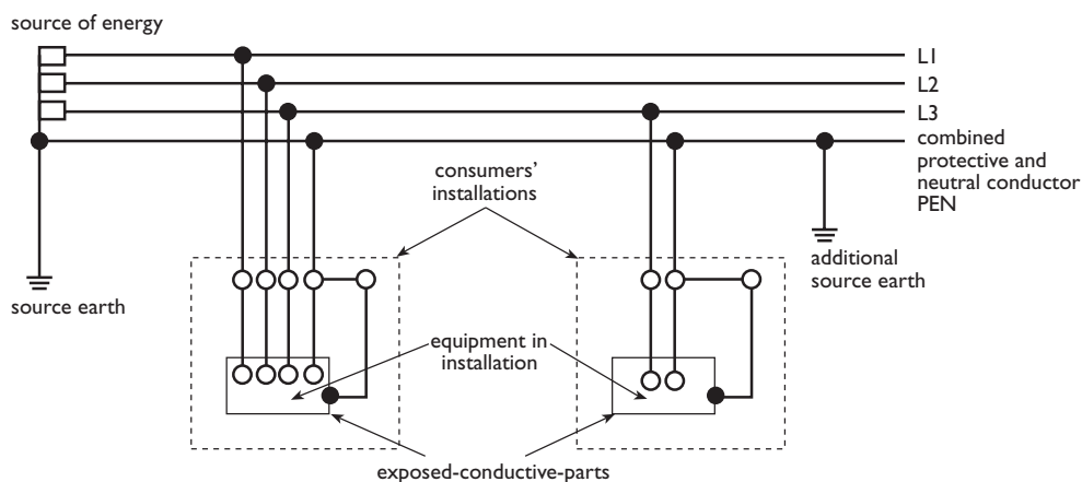
Figure 10 TN-C-S System
