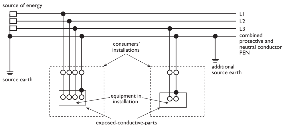
Figure 8 TN-C System
